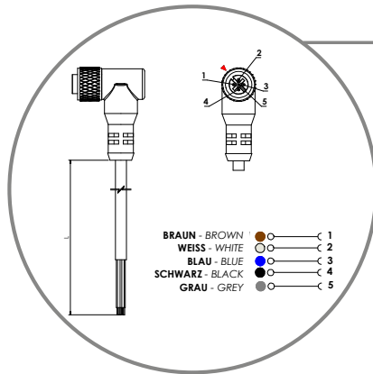
cod. CBL200-002 2 m Kabel mit M12-Verbinder 90° 2 mt cable with connector M12 angled 90°
