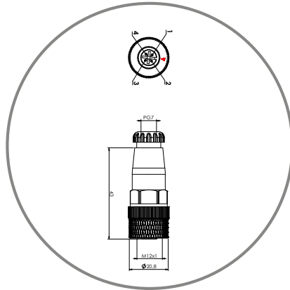
cod. CNN004-006 M12-Verbinder, zu verdrahten M12 connector to be wired
