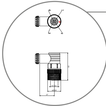
cod. CNN004-007 M12-Verbinder 90°, zu verdrahten M12 connector to be wired angled 90°
